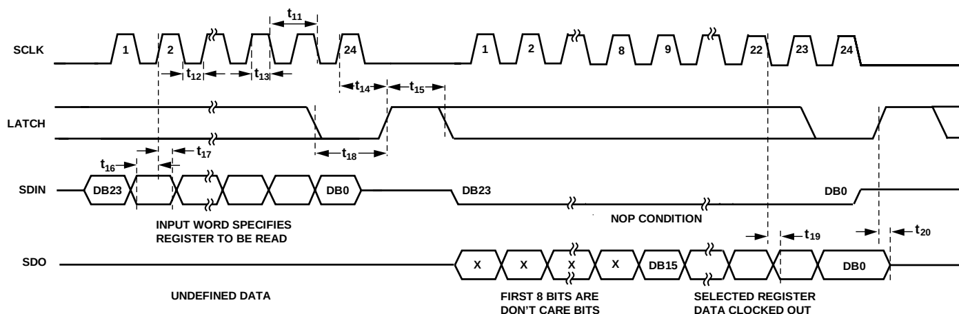
Figure 3. Readback Mode Timing Diagram
