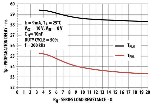
Figure 16. Propagation delay vs. R_g .
