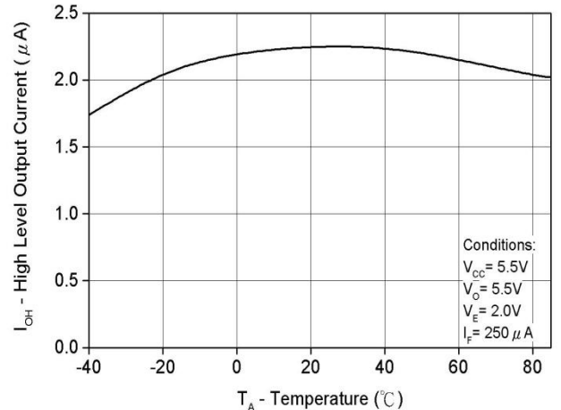
Fig.6 High Level Output Current vs. Temperature
