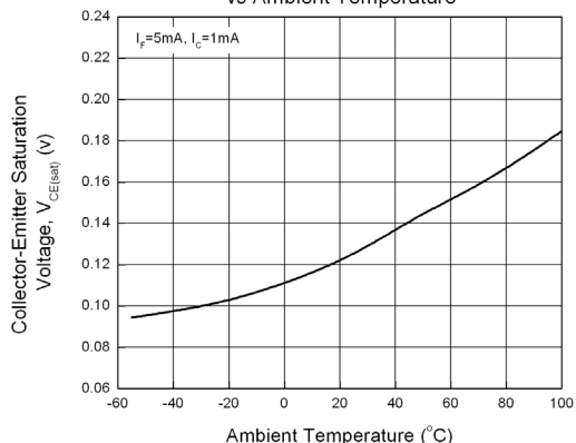
Figure 9. Collector-Emitter Saturation Voltage vs Ambient Temperature
