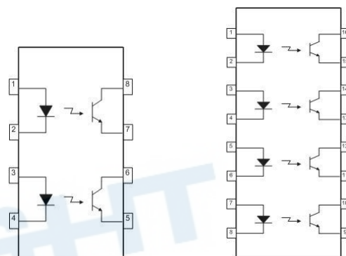
Schematic
