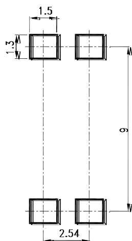
8.1 4 PIN
