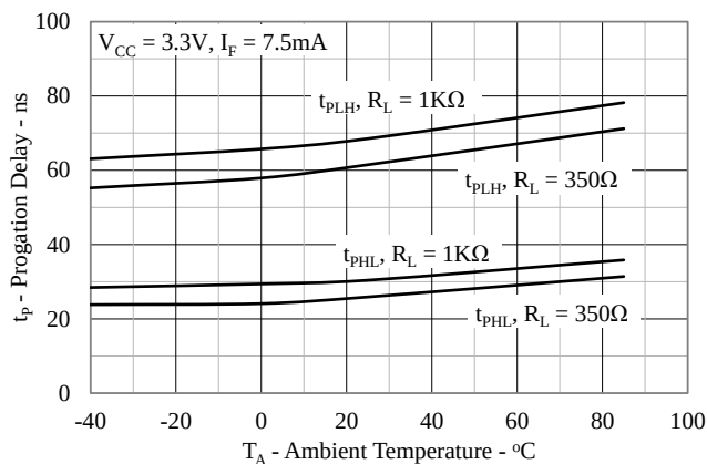
Figure 9: Typical Propagation Delay vs. Ambient Temperature
