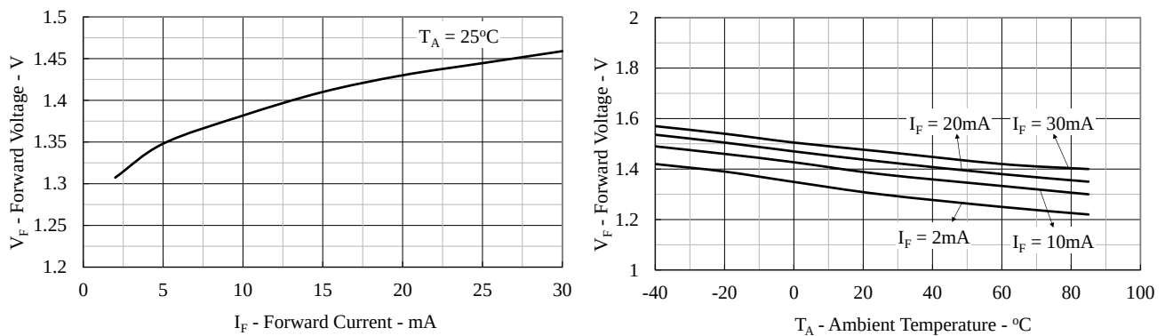
Figure 8: Typical Input Diode Forward Voltage vs. Ambient Temperature
