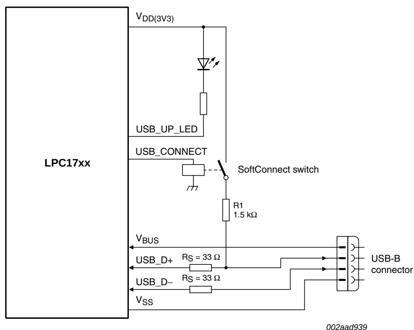
Fig 23. LPC1759/58/56/54/52/51 USB interface on a self-powered device
