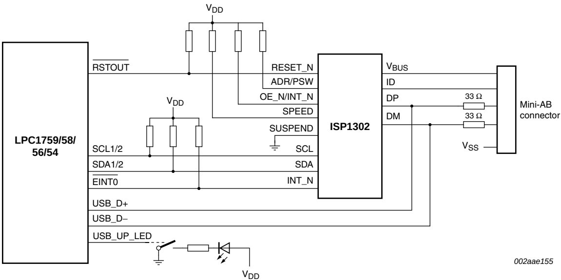
Fig 25. LPC1759/58/56/54 USB OTG port configuration
