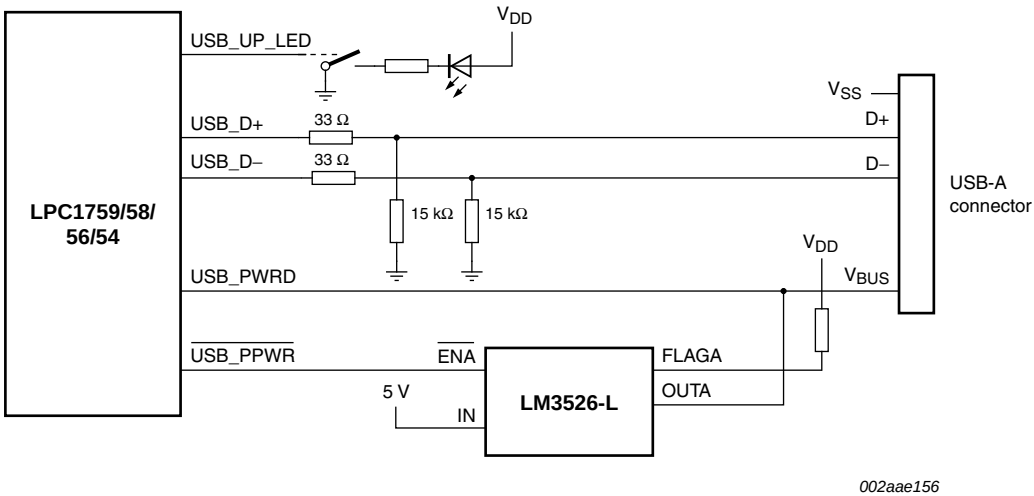
Fig 26. LPC1759/58/56/54 USB host port configuration
