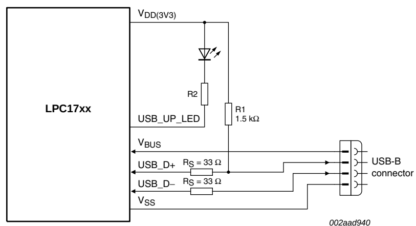
Fig 24. LPC1759/58/56/54/52/51 USB interface on a bus-powered device
