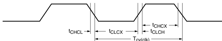
Fig 10. External clock timing (with an amplitude of at least V_{i(RMS)} = 200\text{ mV} )
