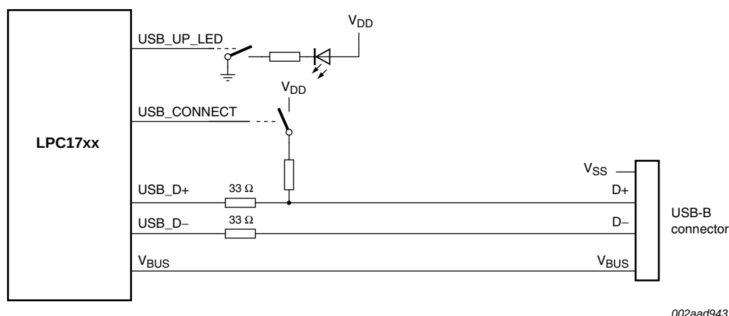
Fig 27. LPC1759/58/56/54/52/51 USB device port configuration
