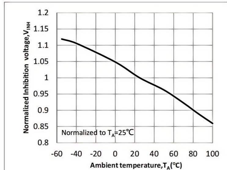
Fig.8 Inhibition voltage vs Ambient temperature
