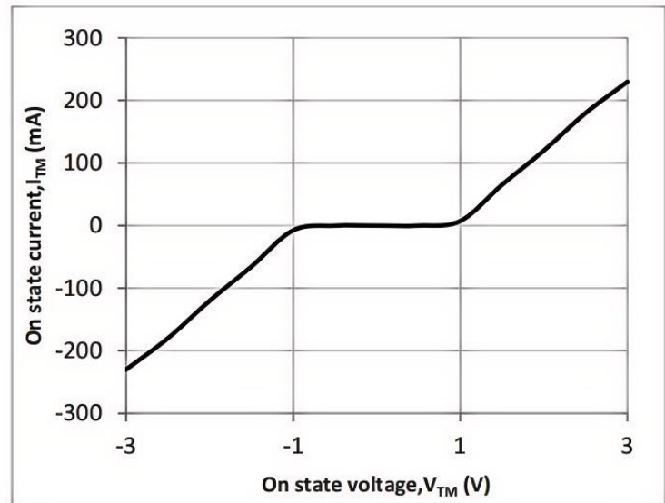
Fig.2 On-state characteristic
