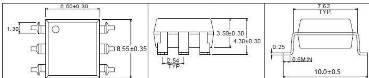
6-pin SMD
