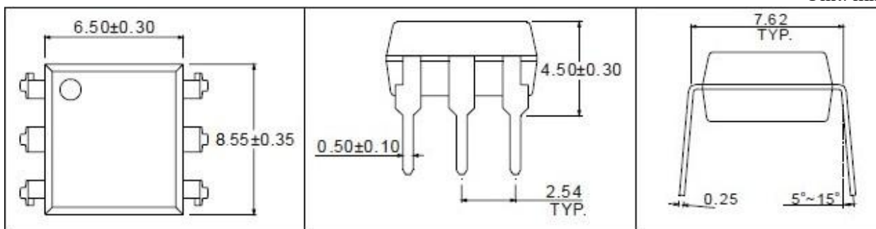
6-pin DIP
