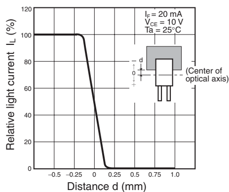
Sensing Position Characteristics (Typical)
