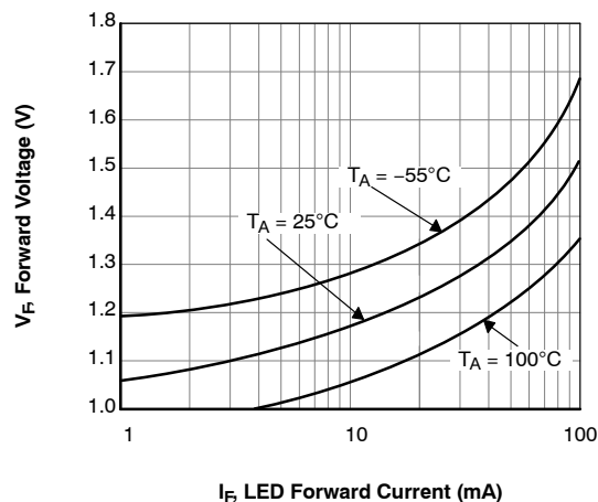
Figure 9. LED Forward Voltage vs. Forward Current
