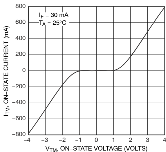
Figure 2. On-State Characteristics
