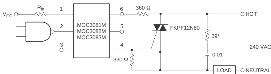
Figure 12. Hot-Line Switching Application Circuit
