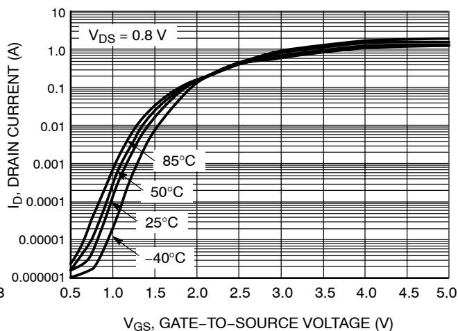
Figure 3. Transfer Function
