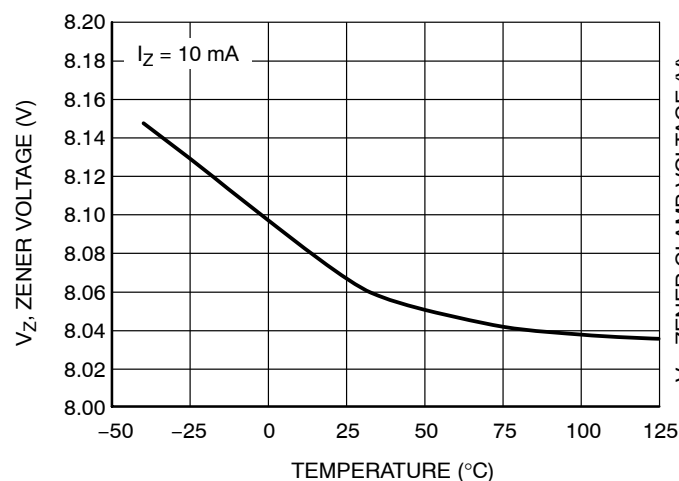
Figure 6. Zener Voltage vs. Temperature
