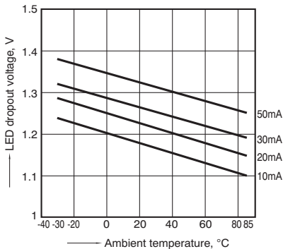
4. LED dropout voltage vs. Ambient temperature characteristics LED current: 10 to 50 mA
