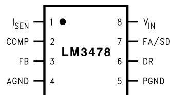
Figure 3. 8-Lead SOIC-8 Package
