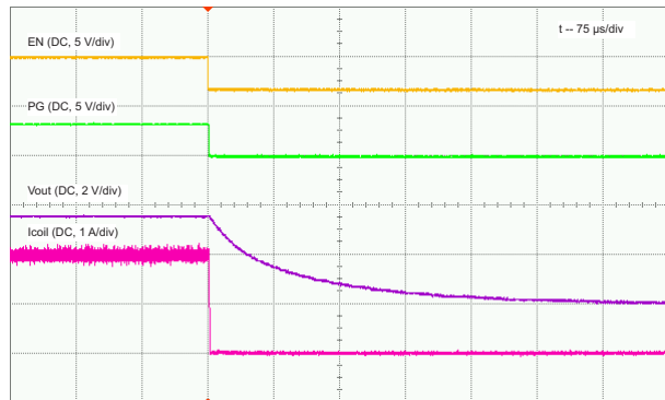
Figure 34. Shutdown ( V_{OUT} = 3.5 \text{ V} , V_{IN} = 3.0 \text{ V} , R_{OUT} = 2.3 \text{ Ω} )
