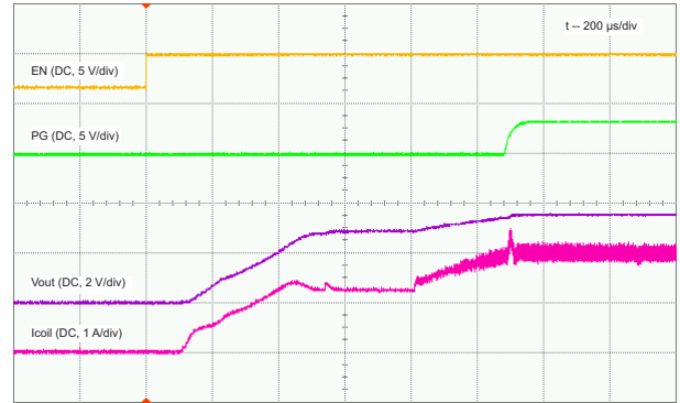
Figure 33. Startup ( V_{OUT} = 3.5 \text{ V} , V_{IN} = 3.0 \text{ V} , R_{OUT} = 2.3 \text{ Ω} )
