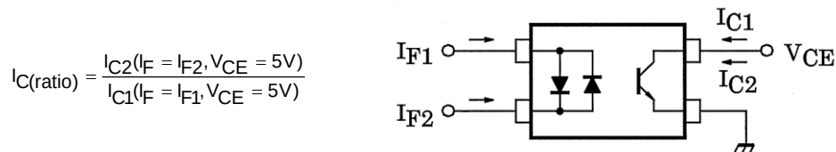
Figure 1: Collector current ratio test circuit
