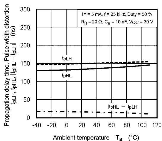
Fig. 13.2.12 t_{pLH}, t_{pHL}, |t_{pHL} - t_{pLH}| - T_a
