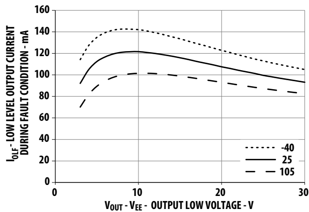
Figure 9. I_{OLF} vs. output voltage
