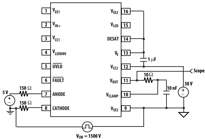
Figure 16. CMR V_{OUT} High test circuit
