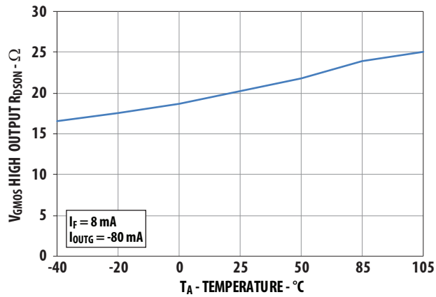
Figure 7. ROUTGH vs. temperature
