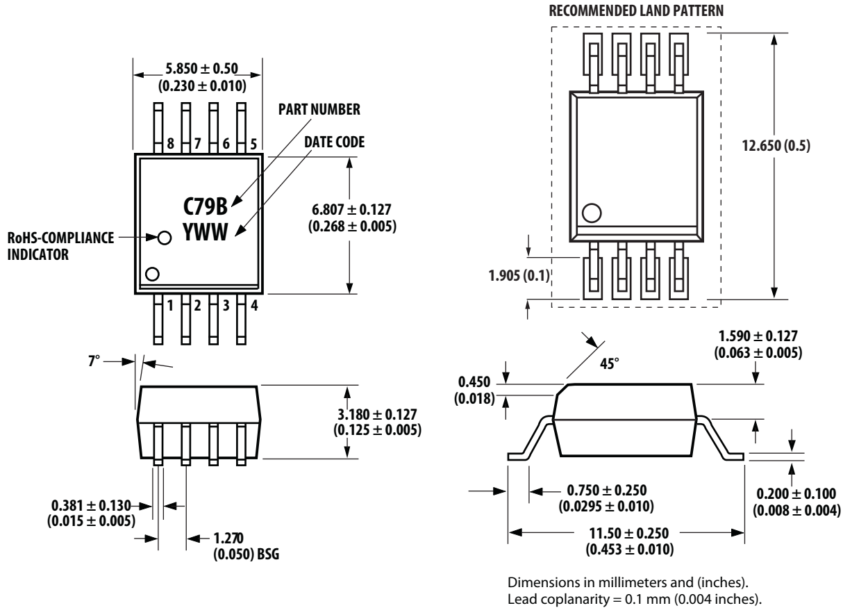
Figure 2. SS0-8 package.
