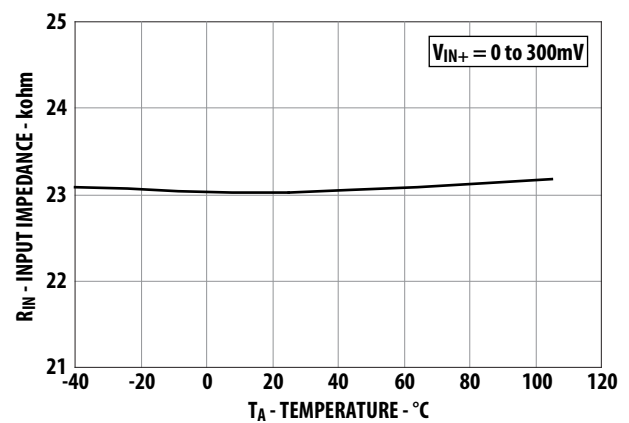
Figure 14. Input impedance vs. temperature.
