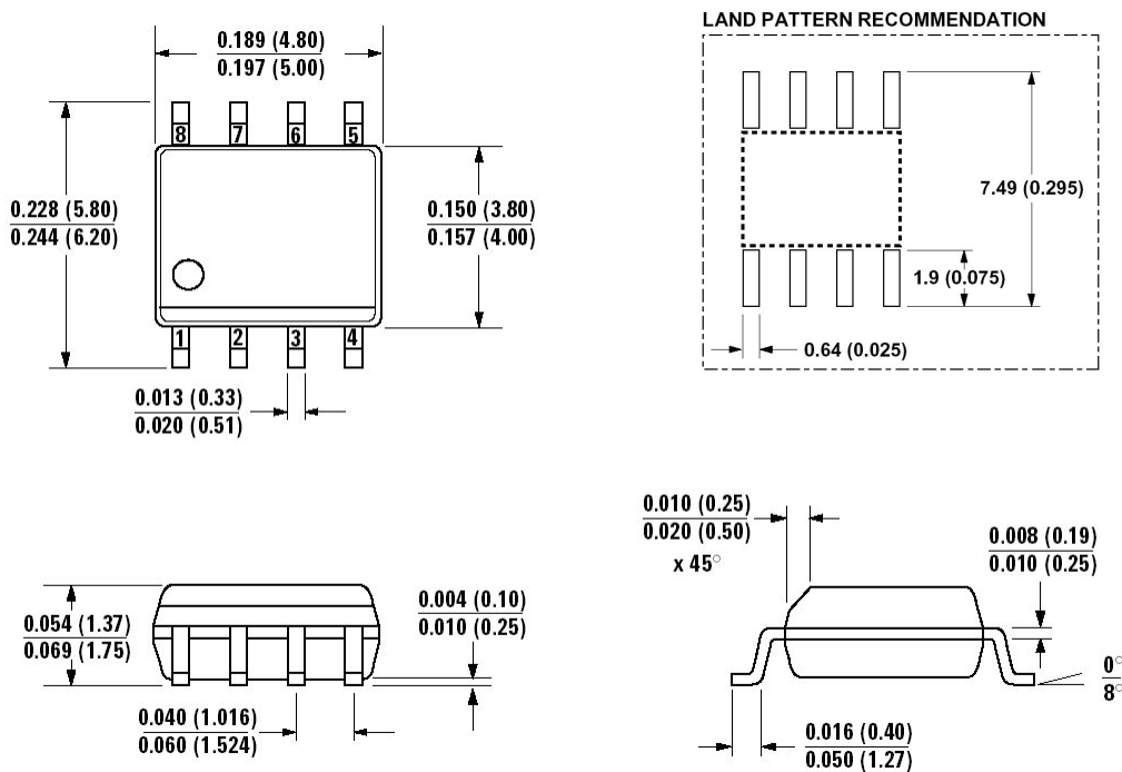
HCPL-0810 Small Outline SO-8 Package
