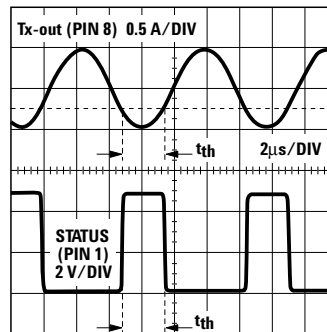
Figure 12. Tx-out load detection.
