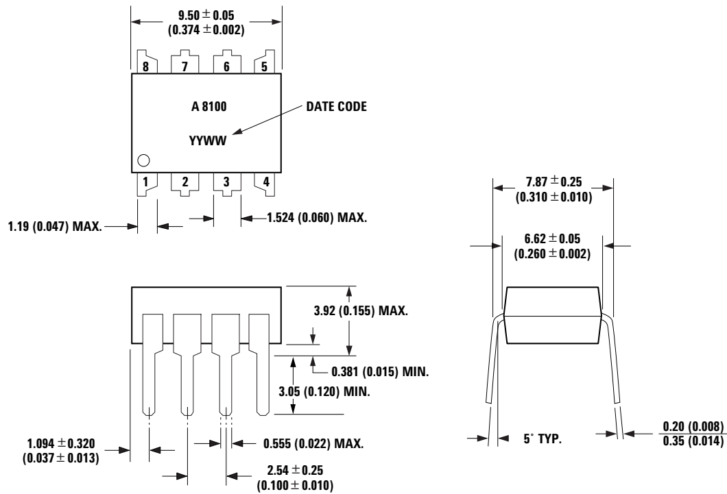
HCPL-8100 Standard 8-pin DIP package
