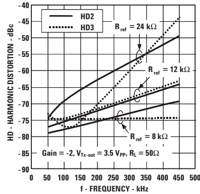
Figure 8. Tx-out harmonic distortion vs. frequency for different values of R_{\text{ref}} at Gain = -2.
