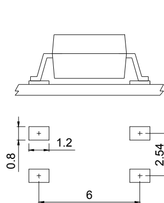
4-pin SOP
