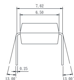
3. Long creepage distance type
