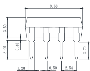
3. Long creepage distance type
