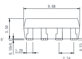
4. Long creepage distance for surface mount type.
