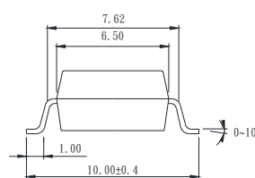
4. Long creepage distance for surface mount type.
