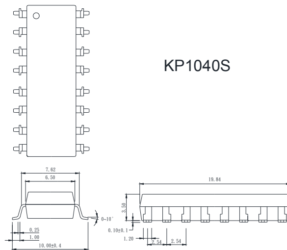
2. Surface mount type.
